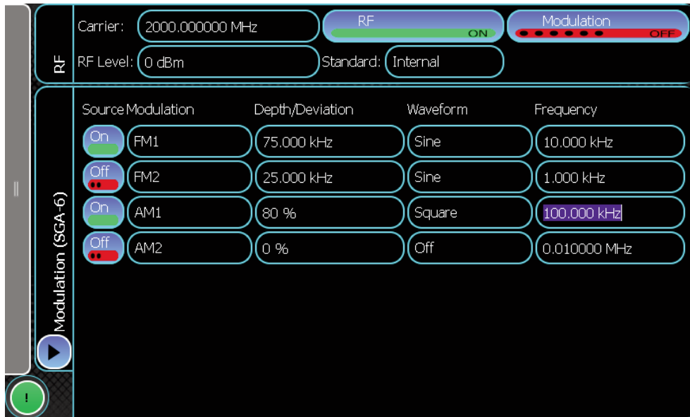
Typical multiple modulation set-up
